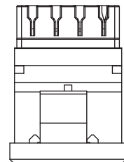
Top view of Category 6 Easy Clip single shielded module
