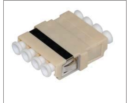
4 port Quad LC Multimode Adaptor, compatible with HellermannTyton Fibre Panels
