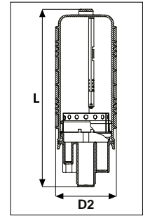
FST 13 Port Closure with Small Hellapon Trays
